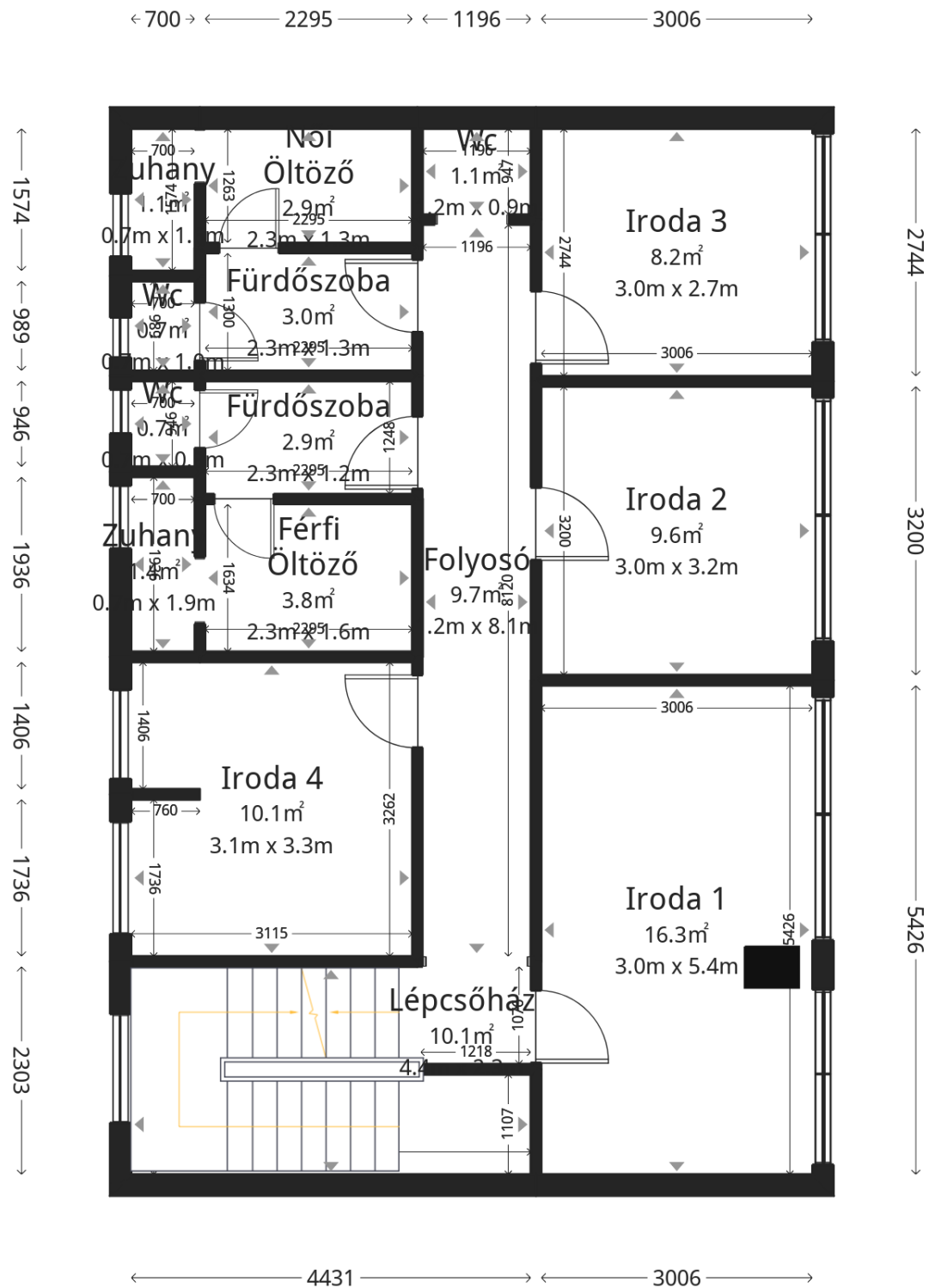
Emelet
